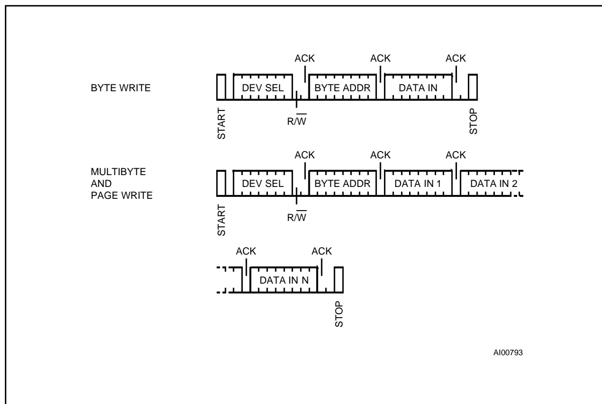
Figure 8. Write Modes Sequence (ST24/25C02)
