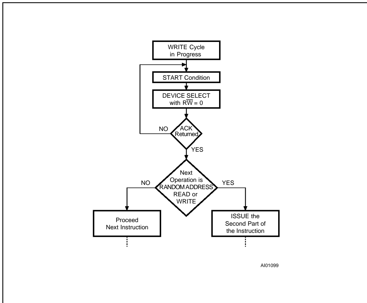
Figure 7. Write Cycle Polling using ACK
